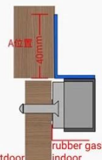
frameless glass door(need U bracket)
