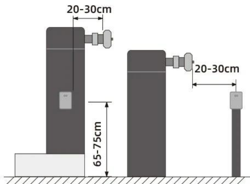
A Gate box with base
