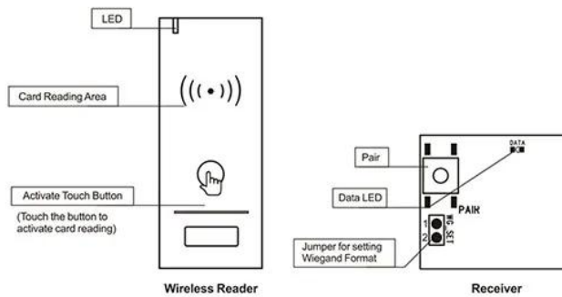
Wireless Reader
