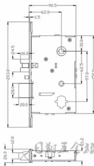
Mortise Size
