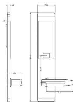
Panel Size
