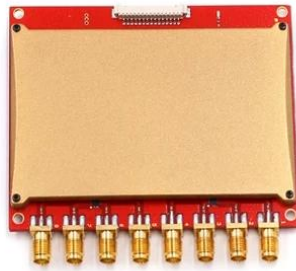
CF-MU808 with eight antenna ports
