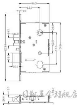
Mortise Size
