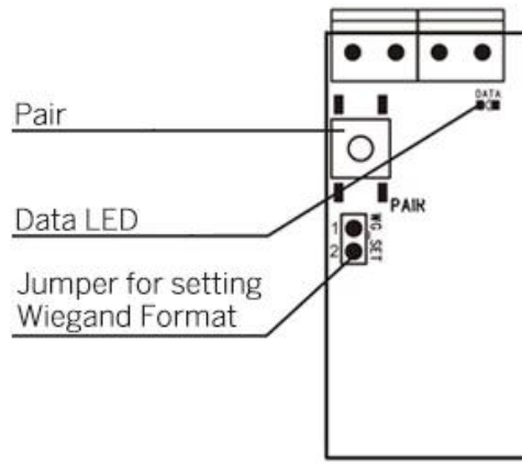
Receiver
