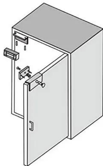
Demonstration of UL Bracket Installation
