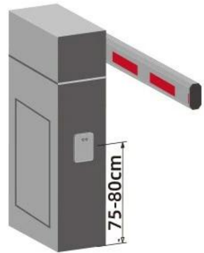
C Gate box without base
