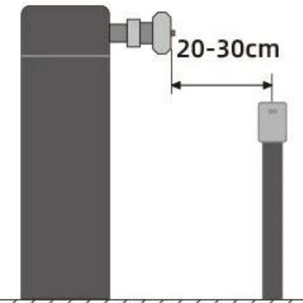
B Gate side column installation
