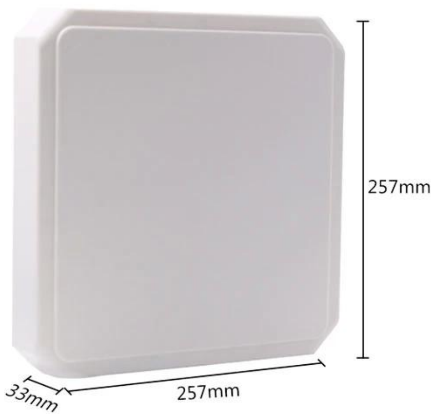
Size:257*257*33mm
