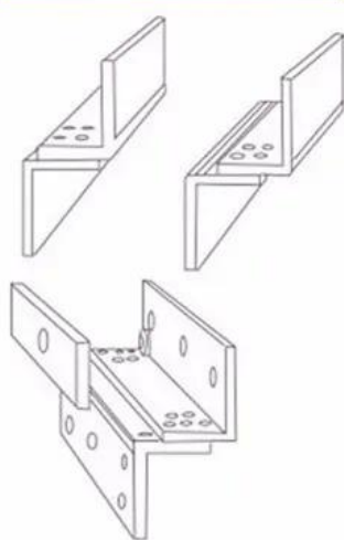
Installation diagram
