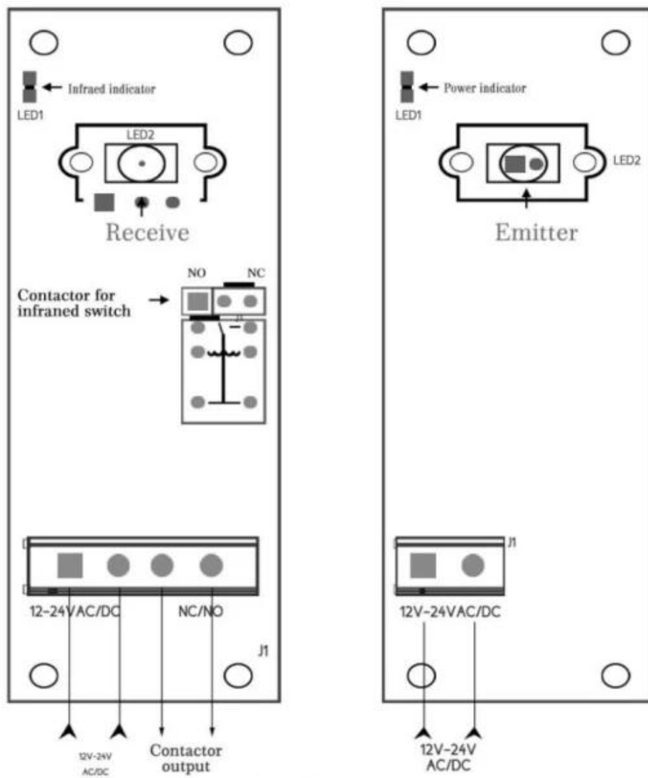
Wiring diagram
