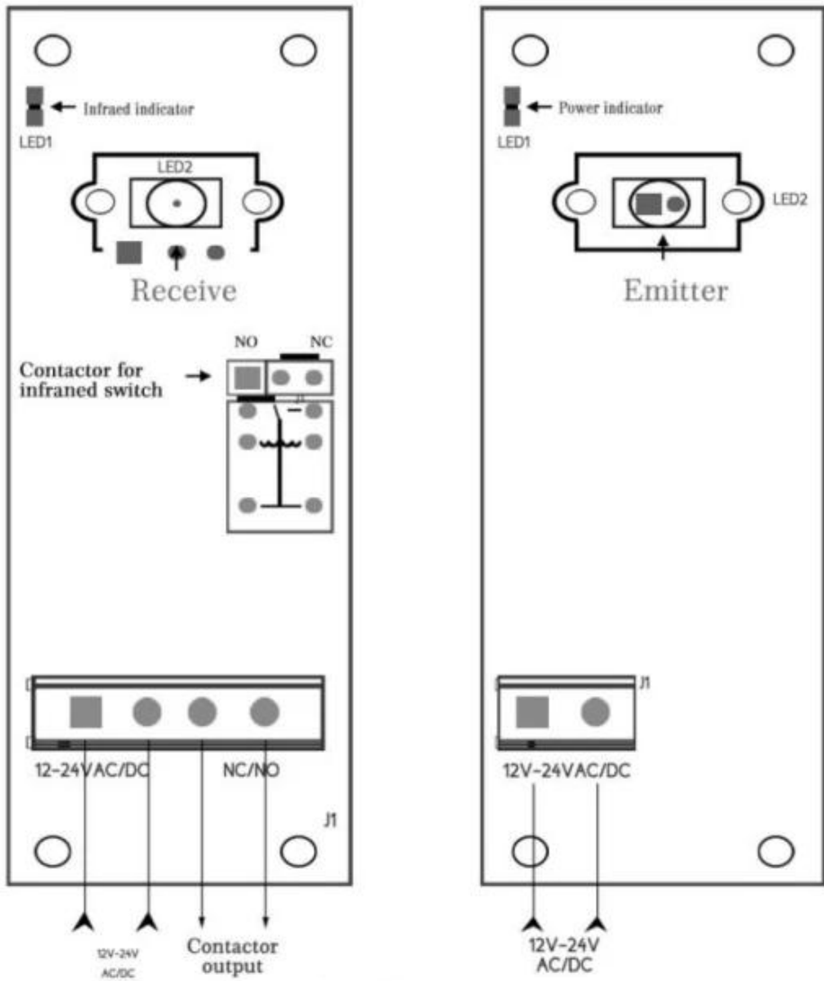
Wiring diagram
