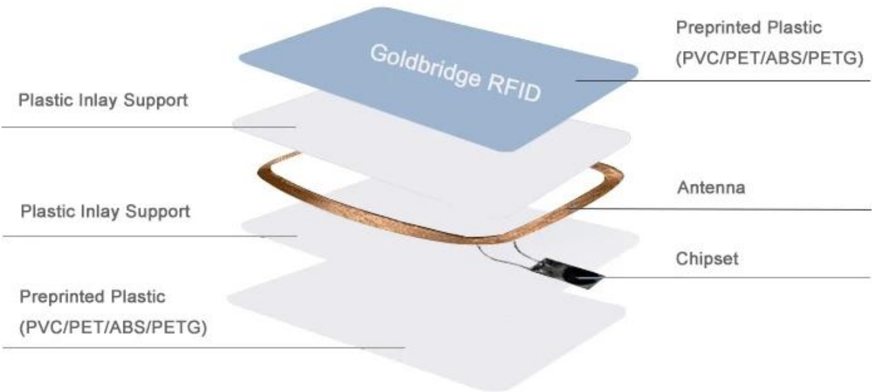
RFID Card Structure
