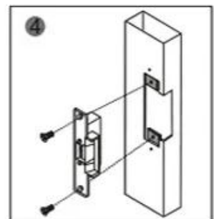
After installed, power on and test it
