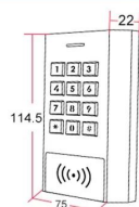
XK1-EM Dimensions: L114.5xW75xD22(mm)
